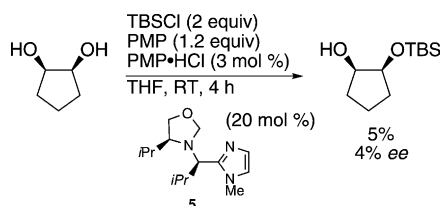
Scheme 3. Control reaction.
